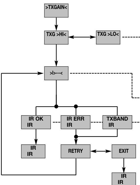
Diagram 8: Setting the audio input gain on the handheld transmitter.
