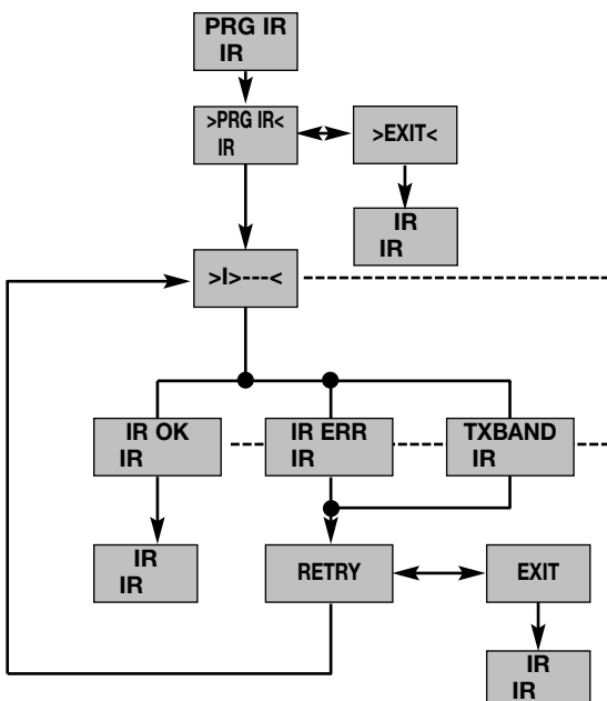
Diagram 7: Setting the transmitter carrier frequency.
