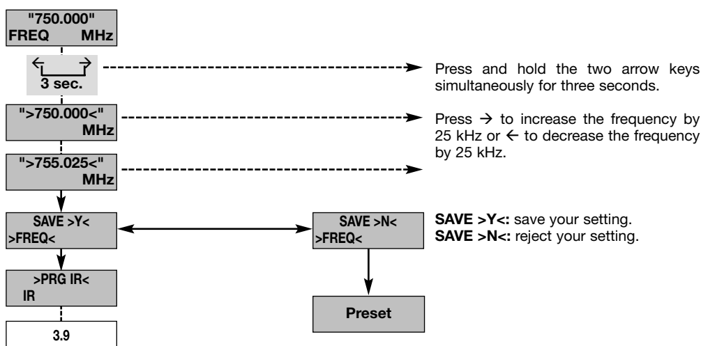
Diagram 5a: Setting frequencies directly.
