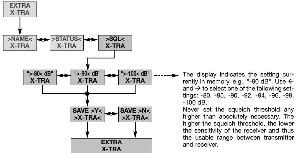
Diagram 10: Setting the squelch threshold.
