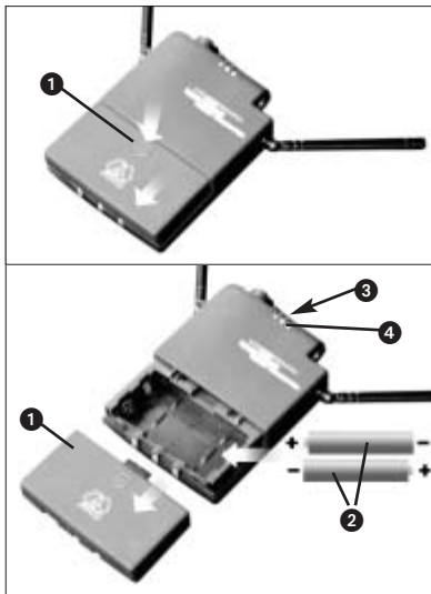
Fig. 3: Inserting batteries.
