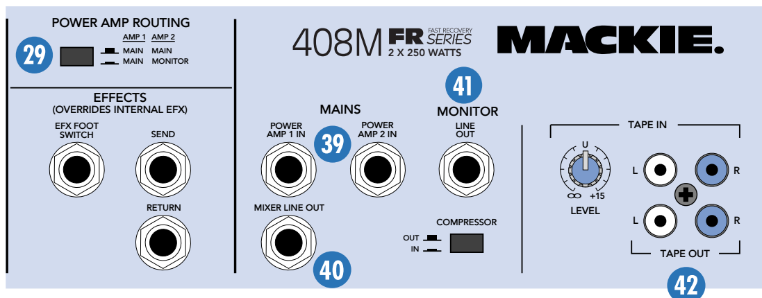
Mono Version Connector Section
