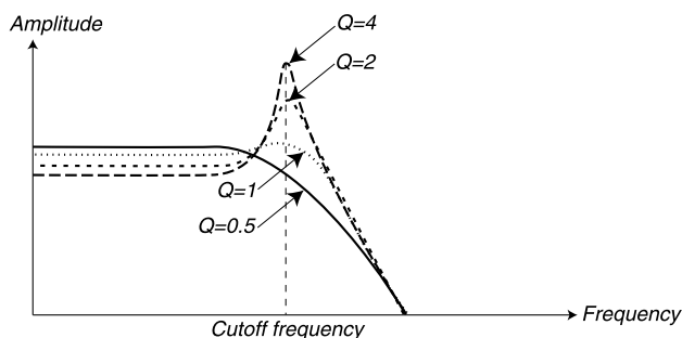
The figure shows a 24 dB lowpass filter with different resonance amounts (Q-values). Q=0.5 represents zero Resonance amount and Q=4 maximum amount.
