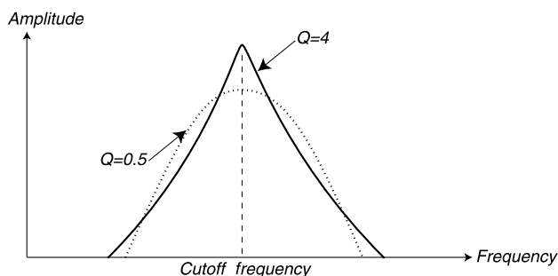
The figure shows a bandpass filter with different resonance amounts (Q-values). Q=0.5 represents zero Resonance amount and Q=4 maximum amount.
