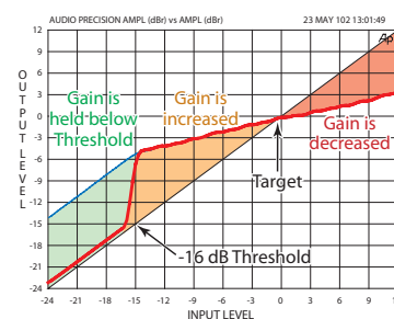
Automatic Gain Control (input level decreasing)
