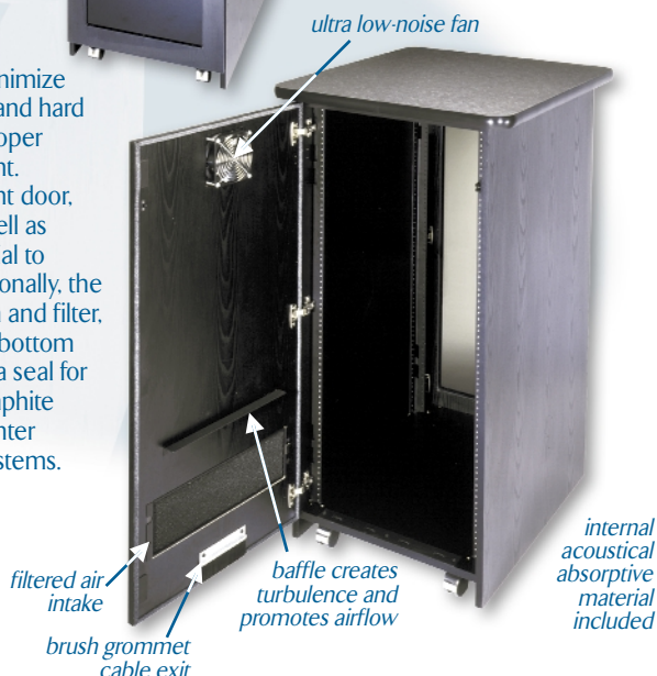
S24DG 24 Space Isolation Rack
