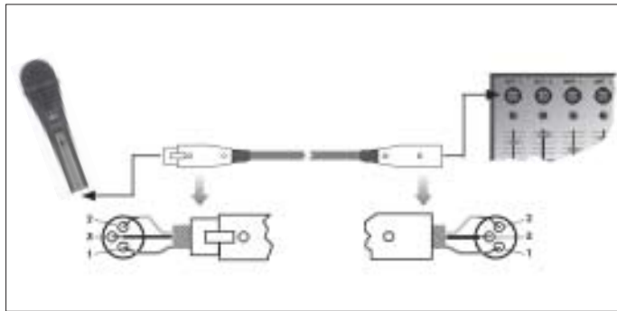
Fig. 4: Using a balanced connecting cable.
