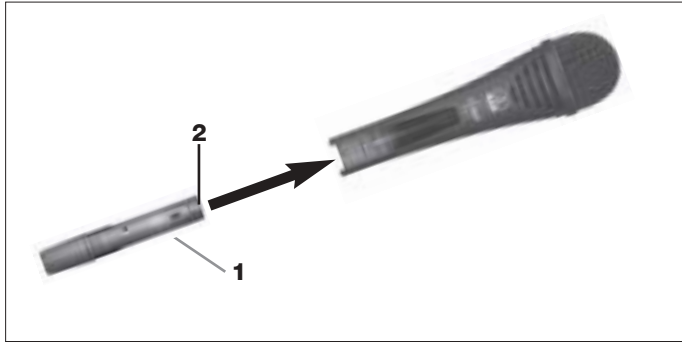
Fig. 7: Installing the transmitter module.
