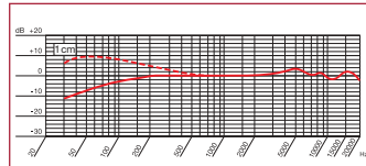
Top chart: Cardioid Bottom chart: Hypercardioid (with PPC 1000)
