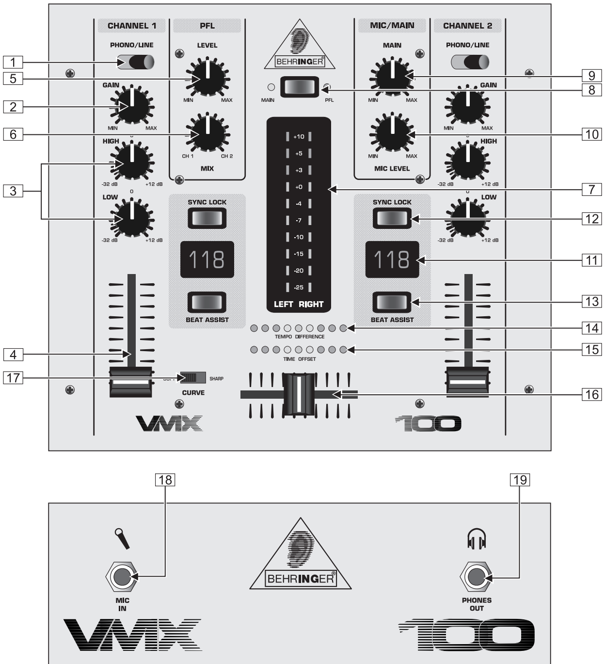
Fig. 2.1 Front view of the PRO MIXER VMX100
