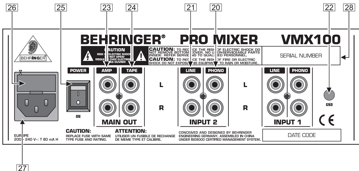
Fig 3.1: Rear view of the PRO MIXER VMX100
