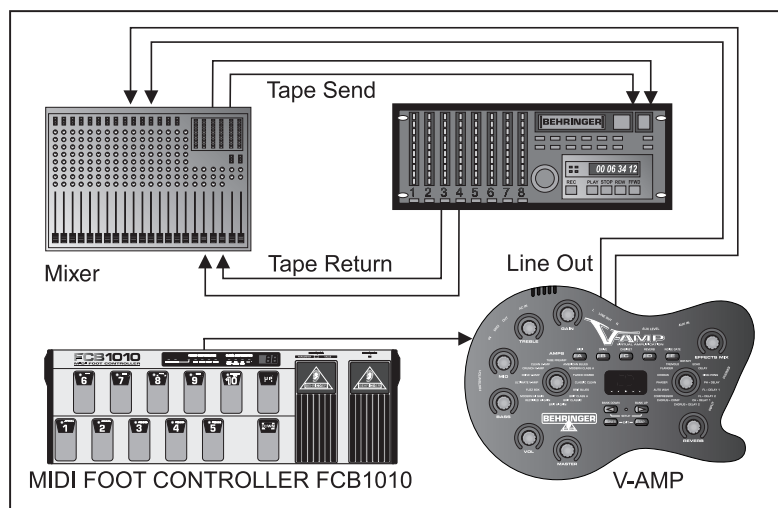
Fig. 2.3: Expanded set-up for studio and home recording applications
