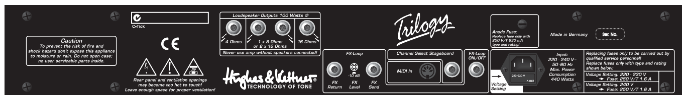
Figure 2: Rear panel
