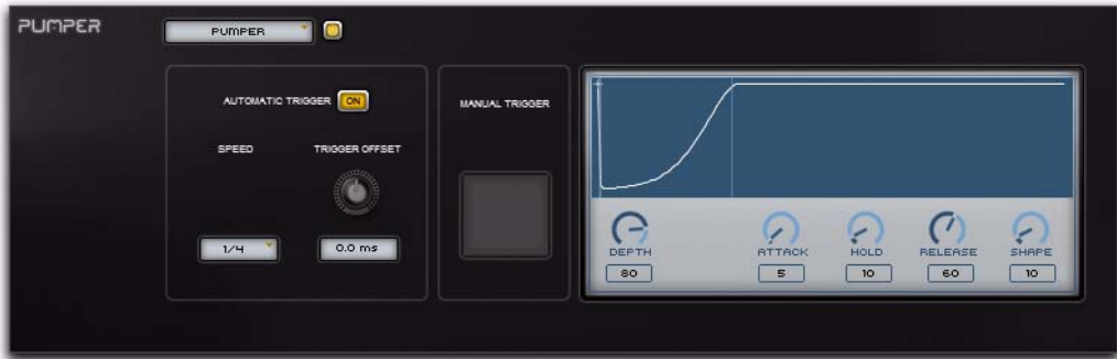
Figure 32. Pumper Editor
