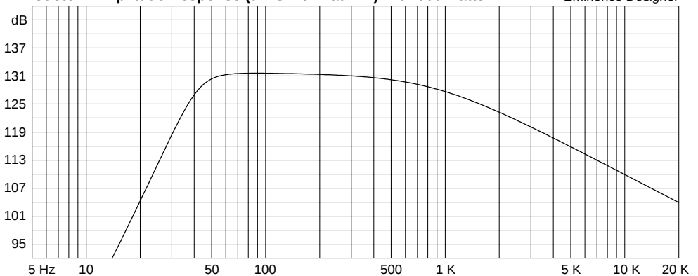
Custom Amplitude Response (dB-SPL/Hz at 1 m) with 900 watts
