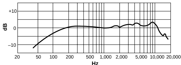
TYPICAL FREQUENCY RESPONSE FIGURE 2
