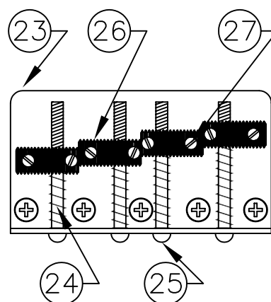
BRIDGE ASSEMBLY
