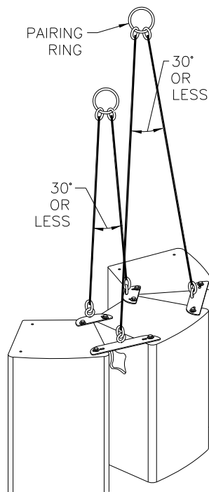
Figure 18: Rigging Three Enclosures with the VFKIT
