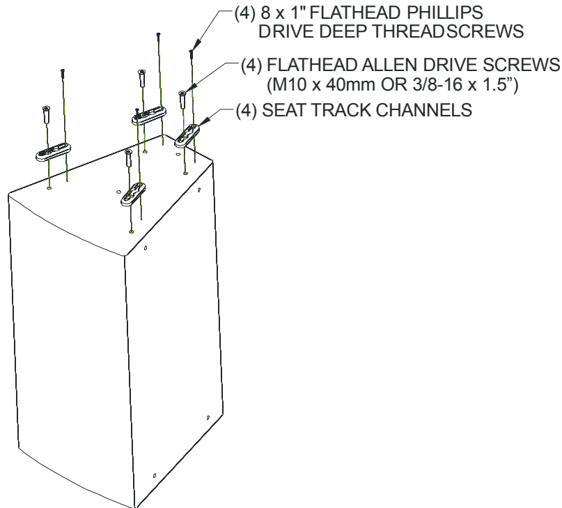
Figure 15: STKIT Assembly of S-Series Enclosure with 4 Seat Track Channels and M10 Hardware
