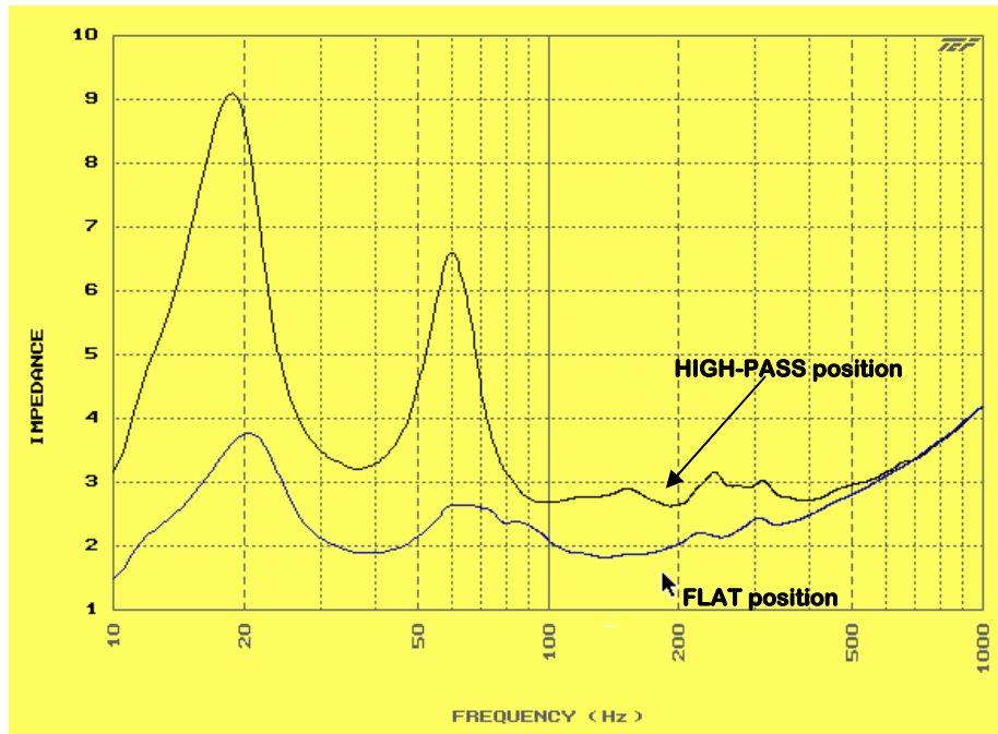
Figure 4: Graph Depicting Response of HIGH-PASS / FLAT Switch
