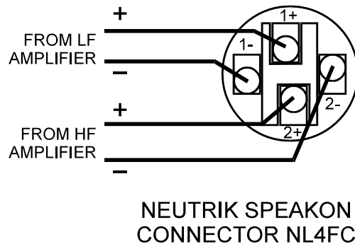
Figure 9: Bi-amp Connections
