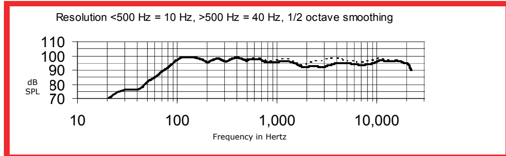
Figure 3: Graph Depicting Frequency Response of MUSIC / VOICE Presence Switch (Note: the Voice/Speech position is represented by the dotted line)
