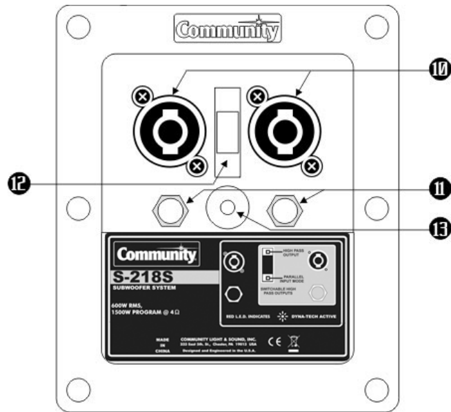
S-Series Subwoofer Input Panel
