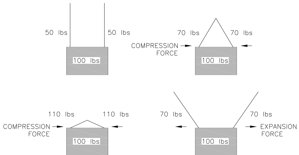
Figure 12: Load Angles
