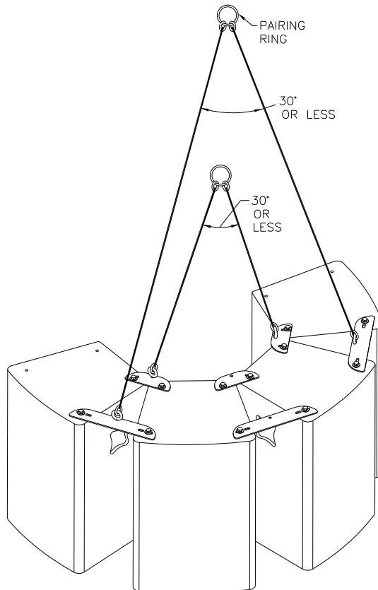
Figure 19: Rigging Four Enclosures with the VFKIT
