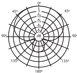
QSNARE Polar Pattern
