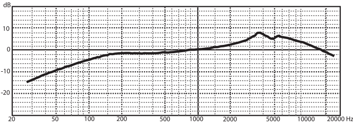
QSNARE Frequency Chart
