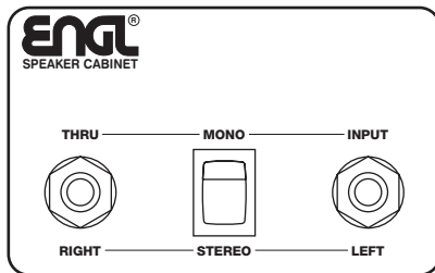
E412 speaker cabinet: rear connection panel
