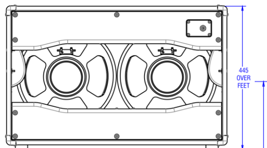
REAR
