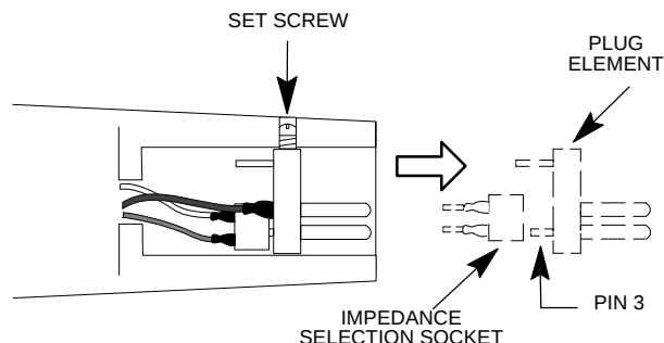
IMPEDANCE SELECTION- RECEPTACLE END OF MICROPHONE
