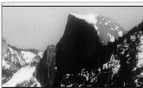
Video window
