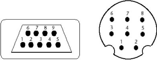
D-Sub 9-Pin Female
