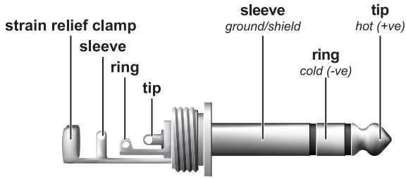
Fig. 4.2: 1/4" TRS connector
