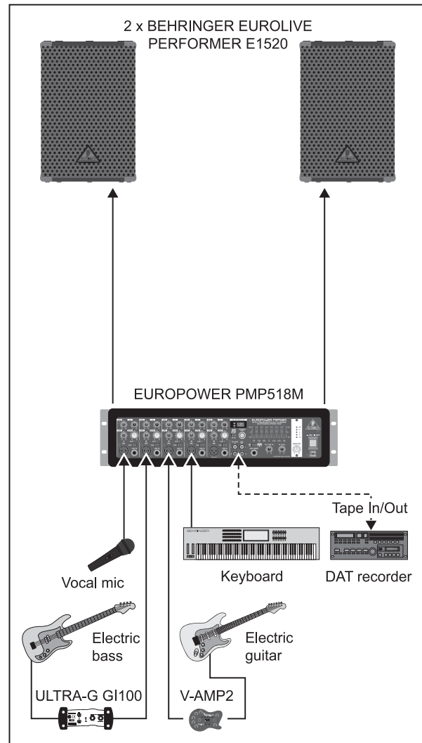
Fig. 5.1: Standard set-up
