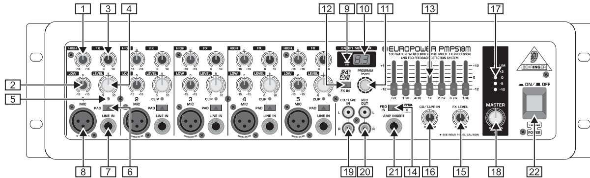
Fig. 2.1: Front panel control elements and connectors
