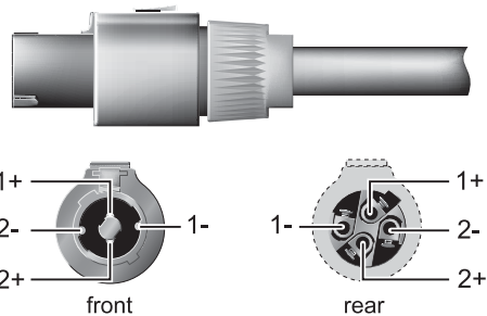
Fig. 4.5: Loudspeaker connector
