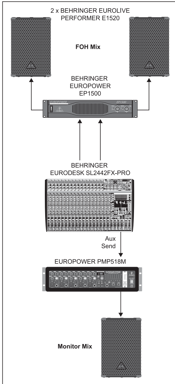
Fig. 5.2: Setup with PMP518M as monitor mixer
