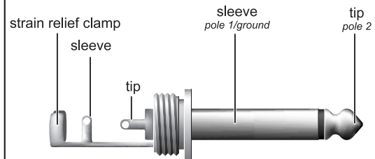
Fig. 4.4: 1/4" mono plug for footswitch
