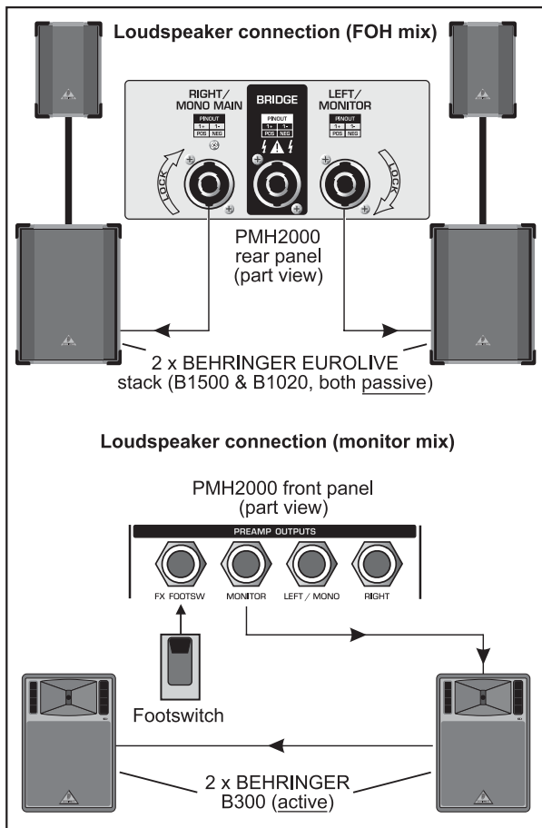
Fig. 5.1: PMH2000 as stereo amplifier (example)
