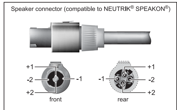
Fig. 4.5: Loudspeaker connector
