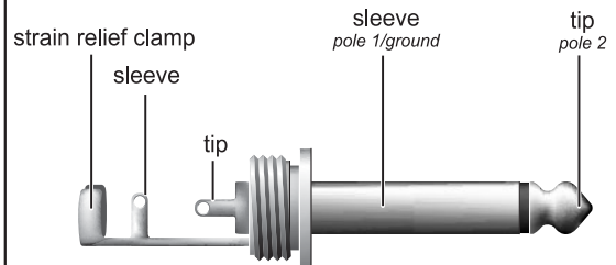
Fig. 4.4: 1/4" TS connector for footswitch
