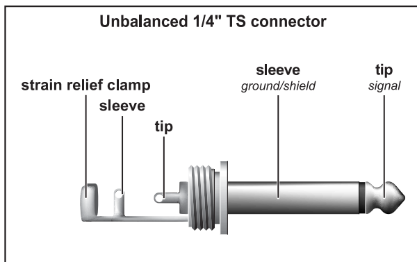
Fig. 4.1: 1/4" mono plug
