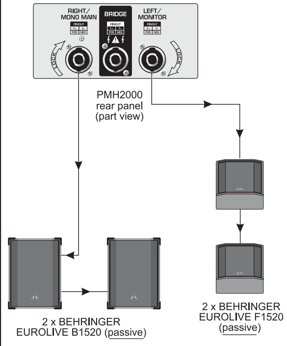
Fig. 5.2: PMH2000 as double mono amplifier (example)
