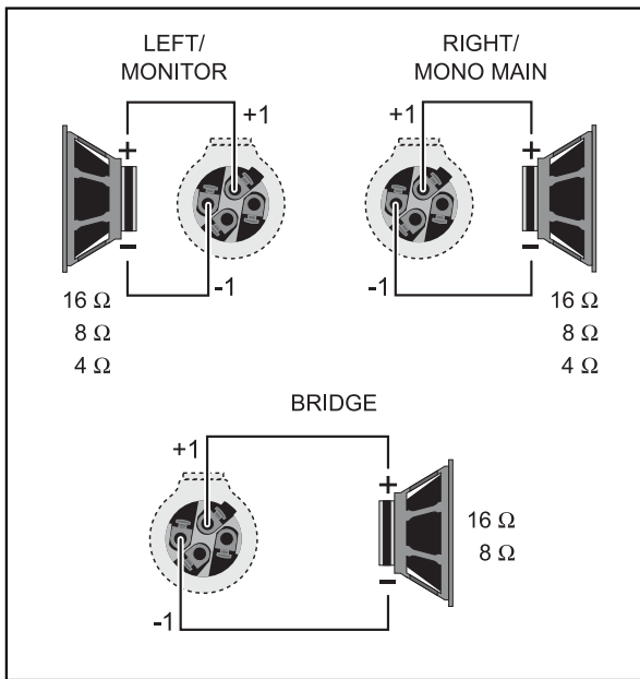
Fig. 4.6: PMH2000 loudspeaker connector assignment
