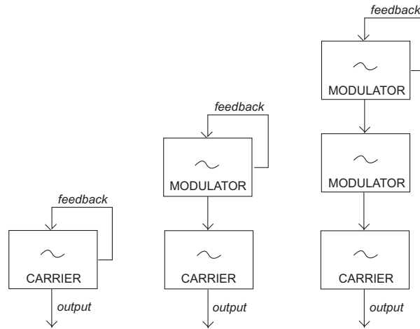
The three different FM algorithms in the Nord Stage: one, two and three oscillator FM with feedback. The feedback is not active in all algorithms.
