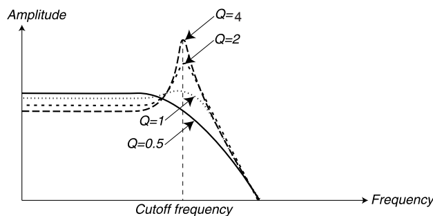
The figure shows a 24 dB lowpass filter with different resonance amounts (Q-values).
