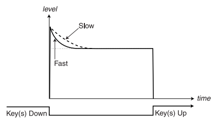
The figure above shows the Percussion envelope in SOFT mode
