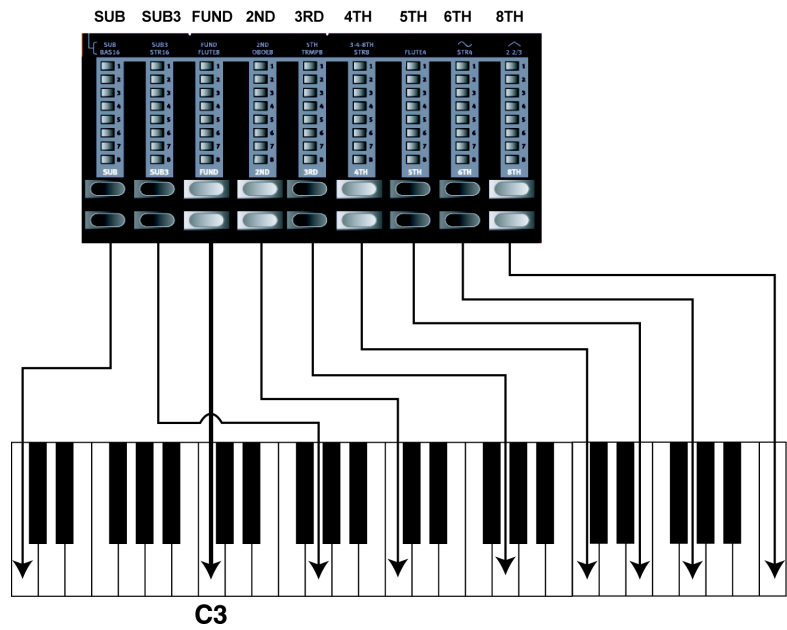
In the figure above we have chosen C3 as our reference note. The FUND drawbar is considered the basic (fundamental) harmonic in the organ sound. The arrows point at the respective note that each drawbar
