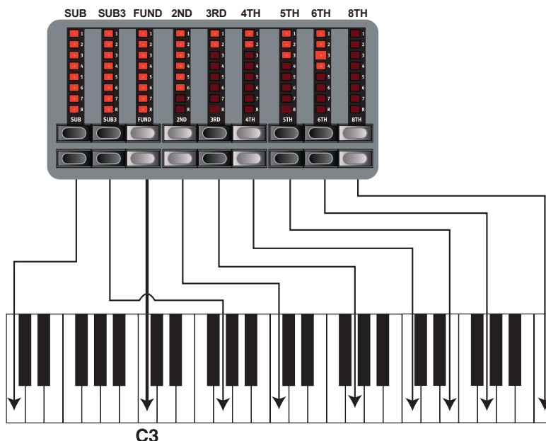
C3 In the illustration above we have chosen C3 as our reference note. The FUND drawbar is considered the basic (fundamental) harmonic in the organ sound. The arrows point at the respective note that each drawbar represents when C3 is our reference note.
