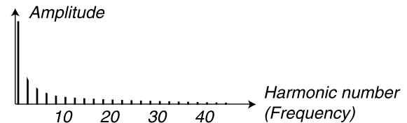
The frequency spectrum of a pure square wave. The signal contains only odd harmonics.
