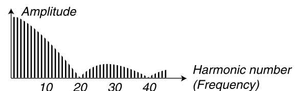
The narrower the pulse width, the more harmonics are present in the frequency spectrum.
