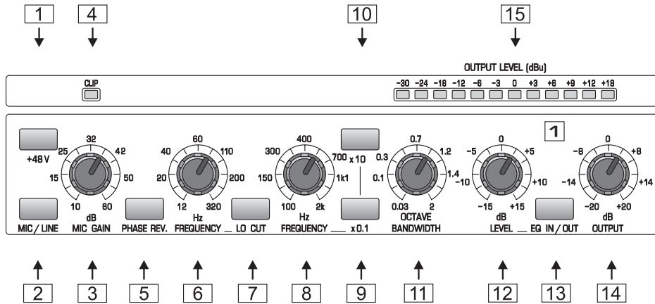
Fig. 4.1: Control elements on the front panel
