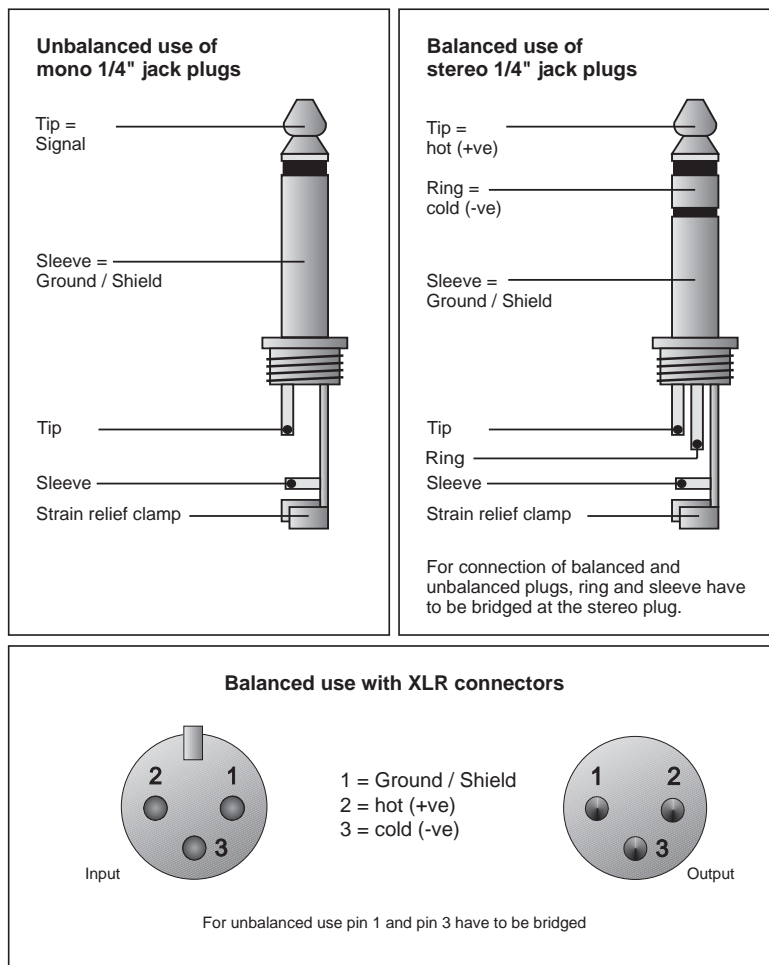
Fig. 3.1: Different plug types
