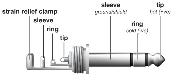
Fig. 8.3: 1/4" TRS connector
