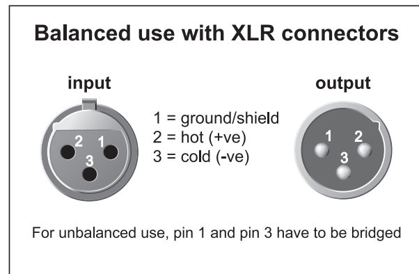
Fig. 5.1: XLR connector
