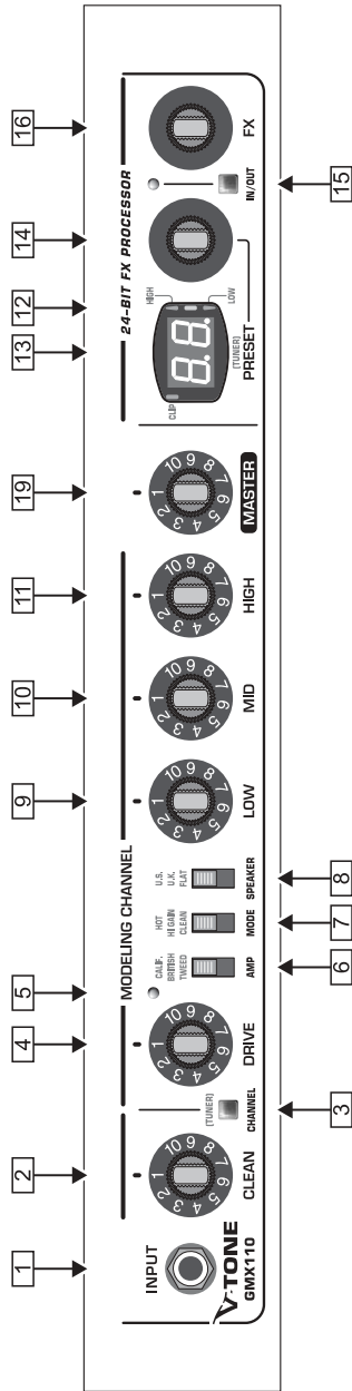
Fig. 1.1: GMX110 controls (front)
