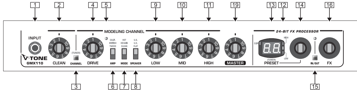
Fig. 1.1: GMX110 controls (front)
