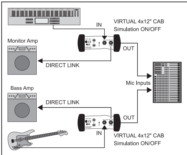
Fig. 2.2: 1. Bass guitar \Rightarrow GI100 \Rightarrow Amplifier/Console 2. Keyboard \Rightarrow GI100 \Rightarrow Amplifier/Console
