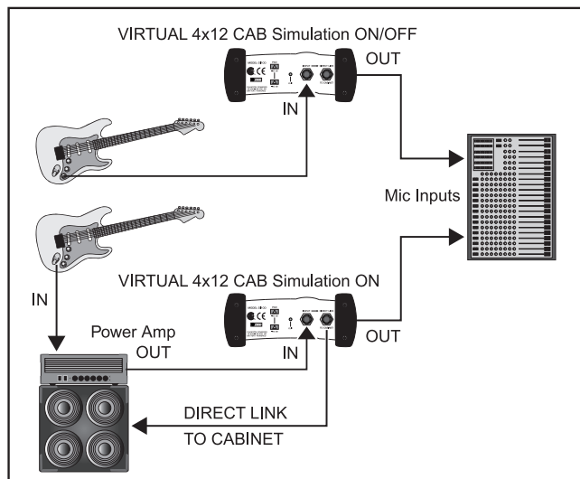
Fig. 2.1: 1. Guitar \Rightarrow GI100 \Rightarrow Console 2. Guitar \Rightarrow Tube amplifier \Rightarrow GI100 \Rightarrow Loudspeaker/Console
