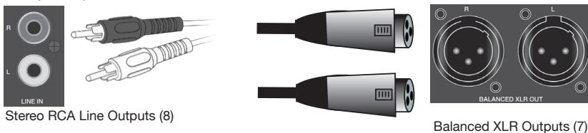
Balanced XLR Outputs (7)
