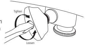
Figure 3: Tuner Tension
