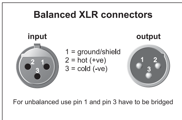
Fig. 4.2: XLR connections
