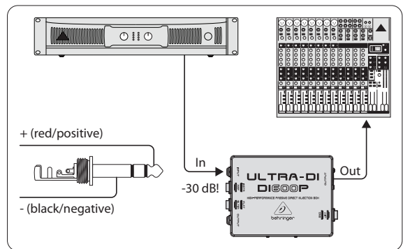
Fig. 3: Connection to a power amp output
