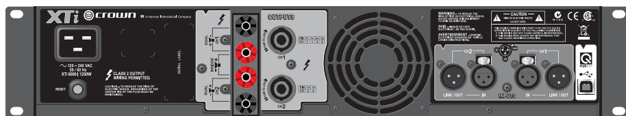
XTi 6000 back panel
