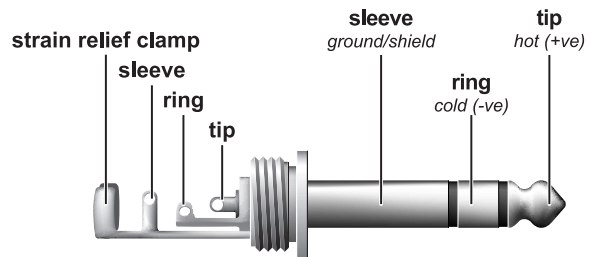
Fig. 4.2: 1/4" TRS connector
