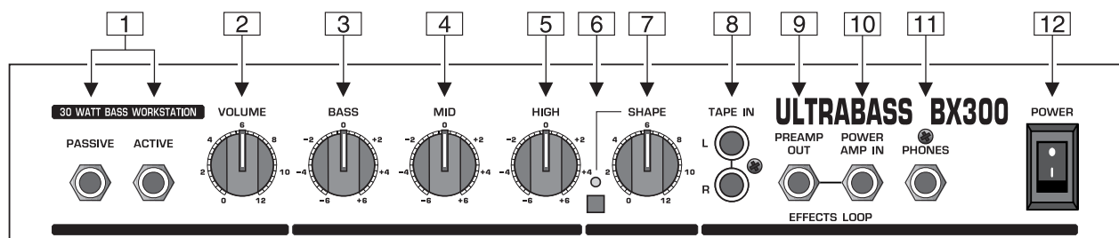
Fig. 1.1: Front panel control elements
