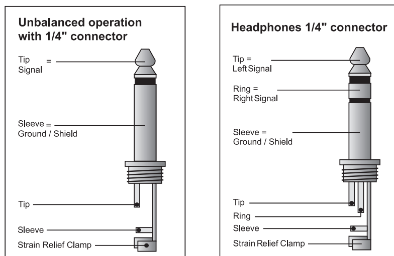
Fig. 4.1: Wiring of mono and stereo (headphones) 1/4" plugs
