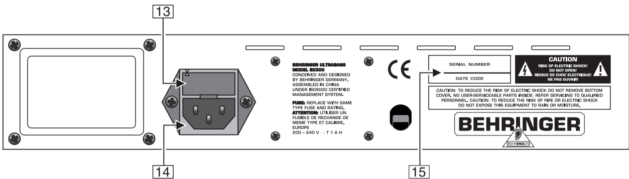
Fig. 1.2: Rear panel connectors
