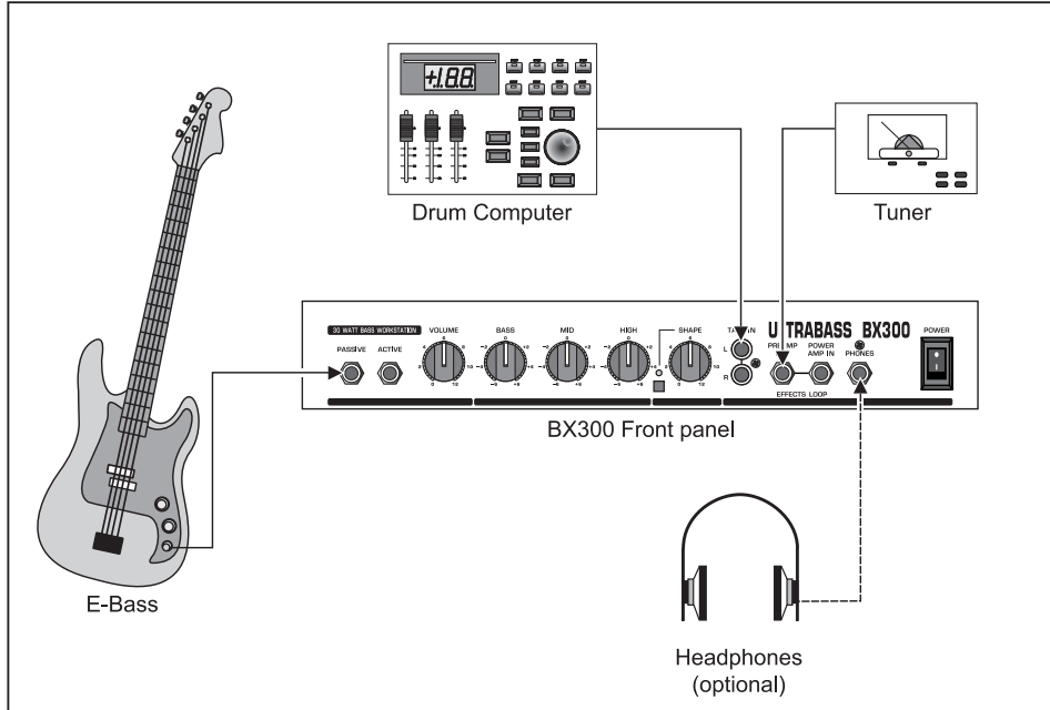
Fig. 2.1: Standard set-up
