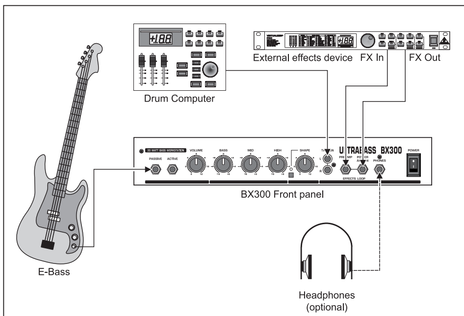
Fig. 2.2: Expanded set-up
