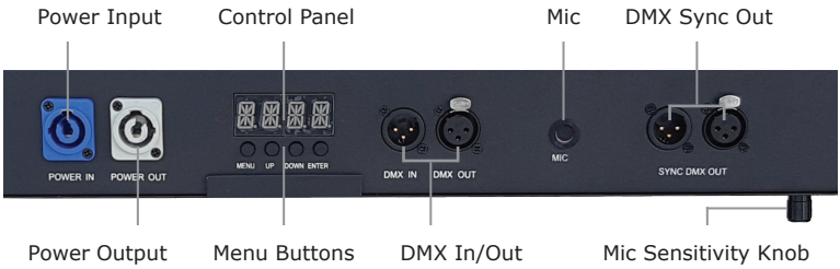
Figure 2: The Rear Connections
