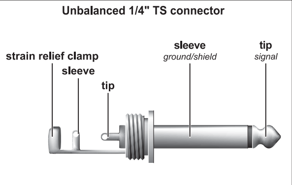
Fig. 6.2: 1/4" TS connector
