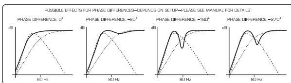
Fig. 3.4: Effect of phase differences on the frequency response
