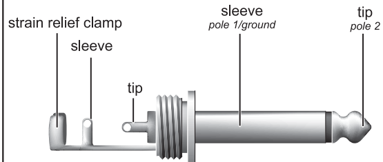
Fig. 4.2: 1/4" TS connector for the footswitch
