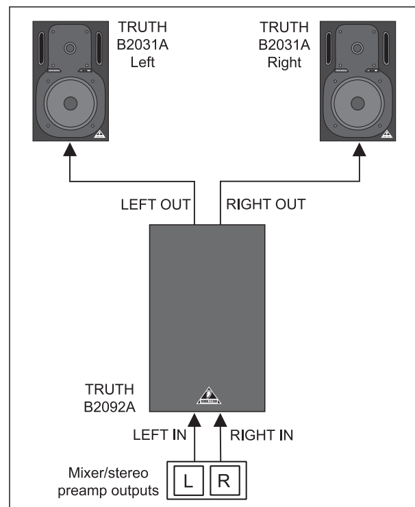
Fig. 3.1: Use in a stereo system
