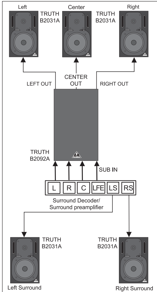
Fig. 3.2: Wiring example for a surround system
