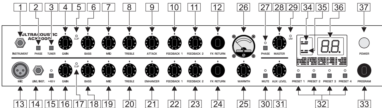
Fig. 1.2: The front panel control elements
